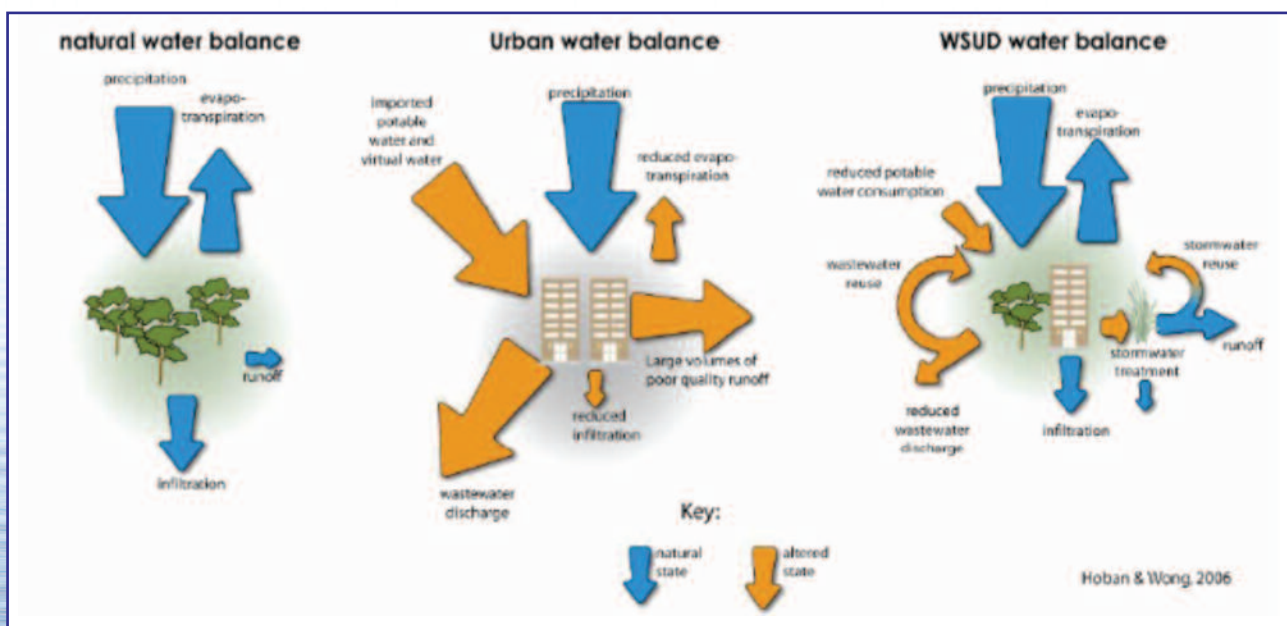
Figure 5.1: Natural water balance
